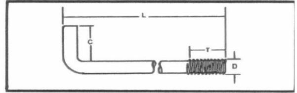
RIGHT ANGLE BENT (DxLxCxT)
